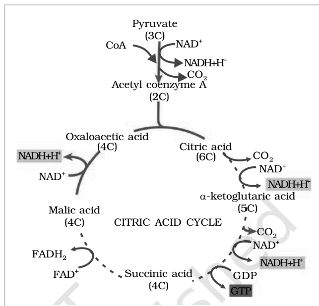
Fig. 12.3 - The Citric acid cycle. Pyruvate (3C) loses \text{CO}_2 and, with CoA and \text{NAD}^+ reduced to \text{NADH} + \text{H}^+ , gives Acetyl coenzyme A (2C) , which condenses with Oxaloacetic acid (4C) to form Citric acid (6C) . Around the ring, decarboxylations give alpha-ketoglutaric acid (5C) and then, via Succinic acid (4C) - the step in which GDP becomes GTP - and Malic acid (4C) , the cycle returns to oxaloacetic acid. \text{FAD}^+ to \text{FADH}_2 marks the single flavin-linked oxidation.
