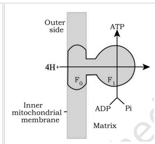
Fig. 12.5 - Diagrammatic presentation of ATP synthesis in mitochondria. The F_1 headpiece projects into the matrix and carries the site where ADP and inorganic phosphate are joined into ATP ; F_0 is the channel through the inner mitochondrial membrane through which 4H^+ return from the intermembrane space down the electrochemical proton gradient for every ATP made.
